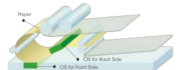
Diagram shows placement of both Contact Image Sensors (CIS) for enhanced scanning speed.
